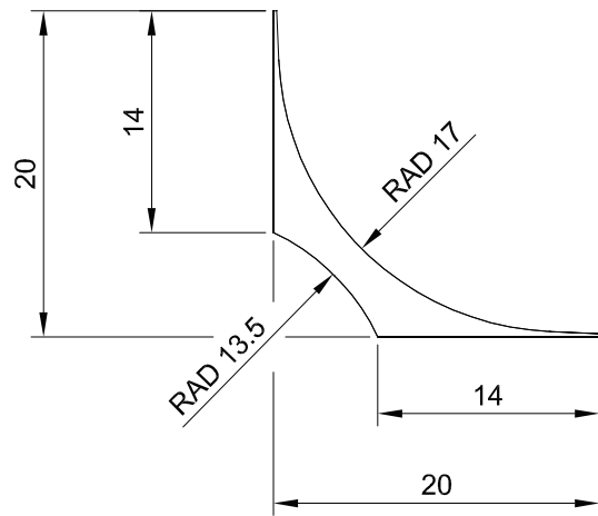
ELEVATION ON PC20- SINGLE PART
