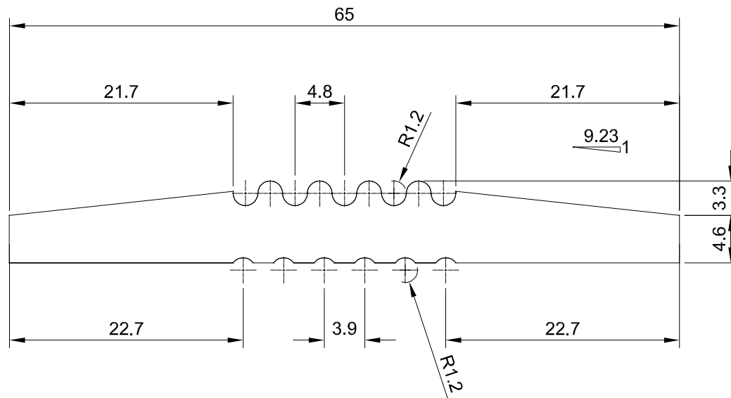
ELEVATION ON EJC65 - SINGLE PART
