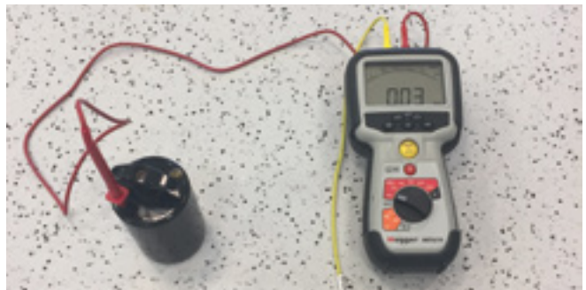
Figure 3 Test electrode with an insulation tester
