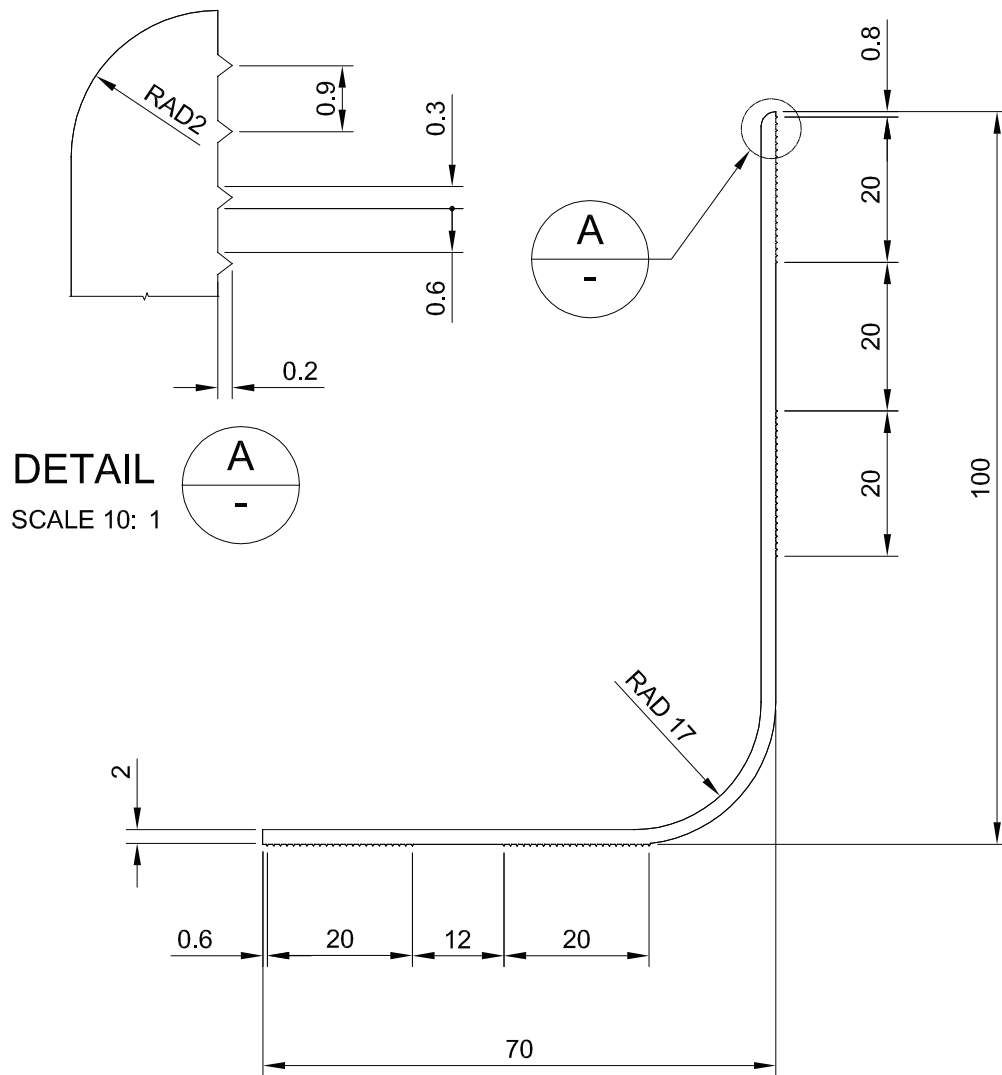
ELEVATION ON MC17C - SINGLE PART SCALE 1:1
